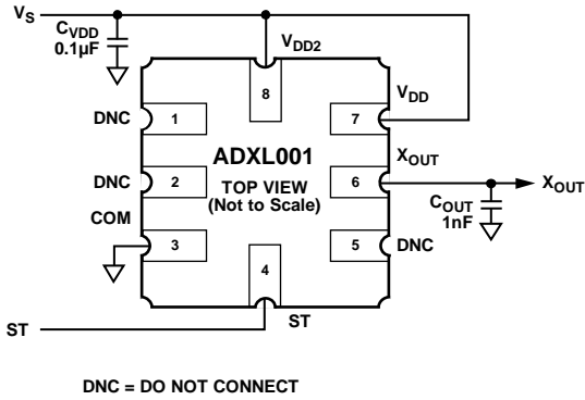
Figure 20. Application Circuit
